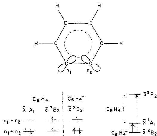
Figure 1. Qualitative illustration of the electronic structure of neutral and anionic o -benzyne. Molecular orbitals labelled n_1 + n_2 and n_1 - n_2 represent the bonding and antibonding combinations, respectively, of the lone-pair-like orbitals relatively localized on the dehydrocarbons. In the singlet ground state of the neutral molecule, the n_1 + n_2 highest occupied orbital is filled, producing a "triple" bond between these carbon atoms. In the present experiment, both the singlet ground state and the lowest triplet excited state of neutral o -benzyne are accessed by photodetachment of an electron from the doublet ground state of the negative ion.
