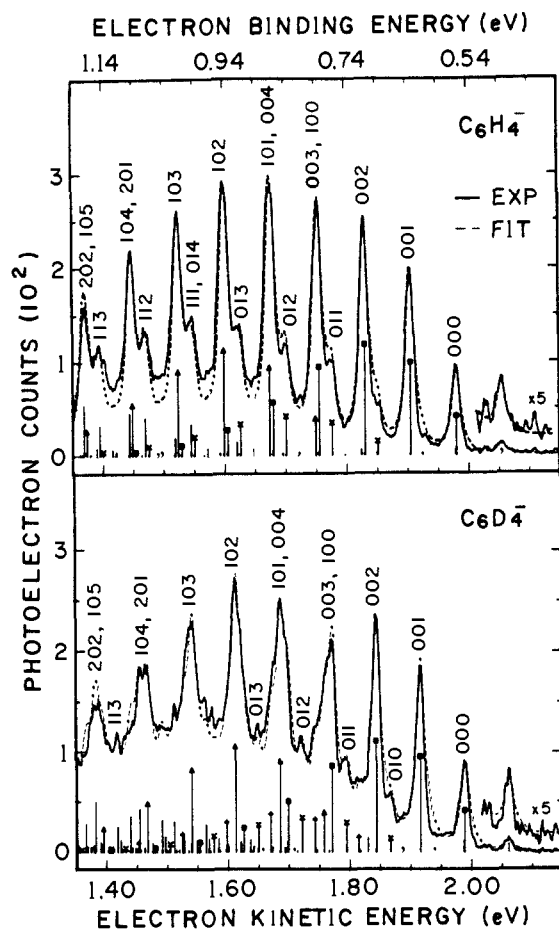
Figure 4. Solid lines show the observed \tilde{X}^1A_1 + e^- \leftarrow \tilde{X}^2B_2 band systems of o -benzyne- h_4 (top) and -d_4 (bottom). Dashed lines show simulated spectra based on a multimode harmonic Franck–Condon fitting to the experimental spectra, for the frequencies and normal mode displacements listed in Table I. Upper-state vibrational assignments for the labeled transitions, all from the zero-point level of the ion, are indicated ( \nu_1' , \nu_2' , \nu_3' ) in order of decreasing intensity. ■ = 00n ( \nu_3' = 605 \text{ cm}^{-1} -h_4 , 585 \text{ cm}^{-1} -d_4 ); × = 01n ( \nu_2' = 1040 \text{ cm}^{-1} -h_4 , 980 \text{ cm}^{-1} -d_4 ); ▲ = 10n ( \nu_1' = 1860 \text{ cm}^{-1} -h_4 , -d_4 ). An additional 00n progression in combination with a fourth mode ( \nu' = 1400 \text{ cm}^{-1} ) is included in the C_6D_4^- simulation (labeled “+”), but this assignment is highly tentative; see text. Insert shows the \nu_3'' = 1 hot band ( 600 \text{ cm}^{-1} C_6H_4^- , 580 \text{ cm}^{-1} C_6D_4^- ), whose intensity indicates an anion vibrational temperature of 300 K.
