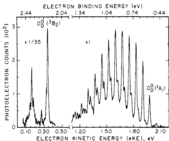
Figure 2. Photoelectron spectrum of the \bar{X}^1A_1 + e^- \leftarrow \bar{X}^2B_2 and \bar{a}^3B_2 + e^- \leftarrow \bar{X}^2B_2 transitions of the o -benzynes anion. Origin bands (labeled 0_0^0 ) observed at electron kinetic energies of 1.980 (10) and 0.343 (15) eV determine the electron affinity and singlet-triplet splitting of neutral o -benzynes. Spectra were obtained with the 488 and 458 nm Ar II laser lines for the singlet and triplet band systems, respectively; for clarity, both portions of the spectrum are drawn as for 488-nm (2.540 eV) excitation.
