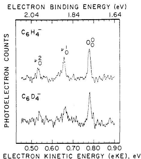
Figure 3. Band systems due to minor \text{C}_6\text{H}_4^- and \text{C}_6\text{D}_4^- isomers, tentatively assigned as m - or p -benzynes anions. These bands were typically about 2% as intense as the triplet o -benzynes system. The observed origin band ( 0_0^0 ) positions correspond to electron binding energies of 1.761 (15) eV for \text{C}_6\text{H}_4^- and 1.759 (15) eV for \text{C}_6\text{D}_4^- . Since transitions to lower energy states may be hidden beneath the stronger o -benzynes bands, these values provide upper limits for the electron affinities. The active vibrational progression has upper state intervals of 980 (30) \text{cm}^{-1} for \text{C}_6\text{H}_4^- and 960 (40) \text{cm}^{-1} for \text{C}_6\text{D}_4^- .
